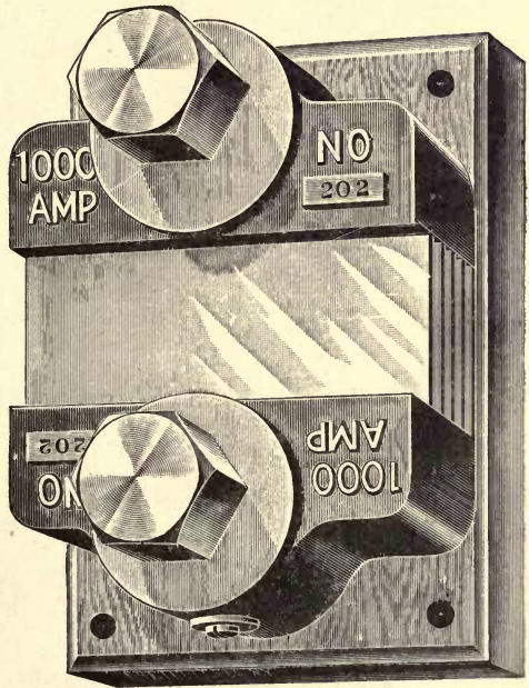
Fig. 125.—Weston 1000 Amp Low-Resistance Shunt for Ammeter
